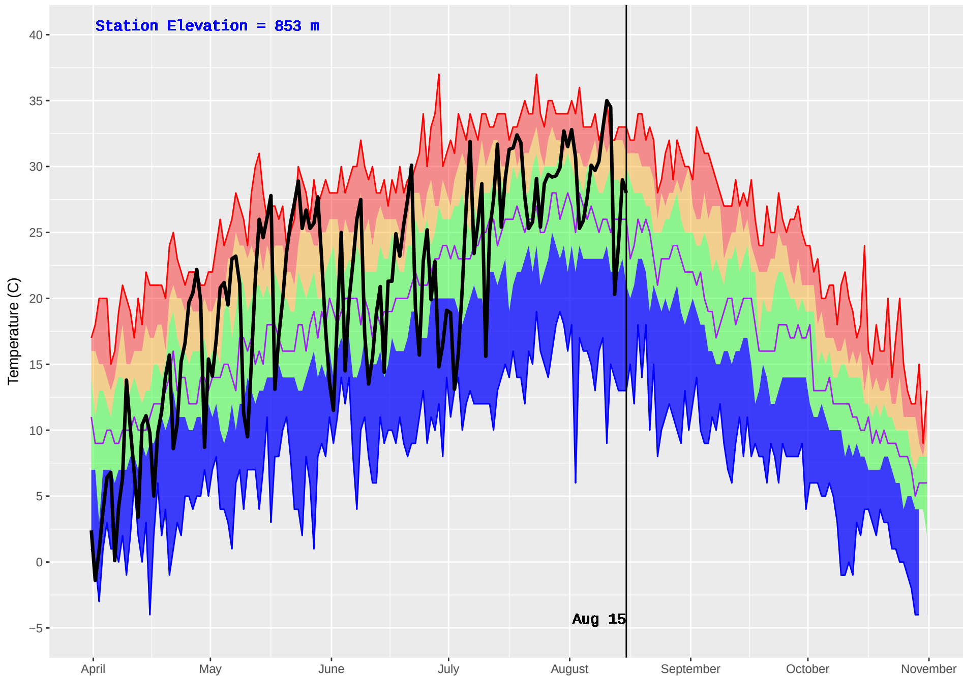
JOHNSON LAKE (419) : Historical (1986–2016) and Current (2018) Daily Temperature
