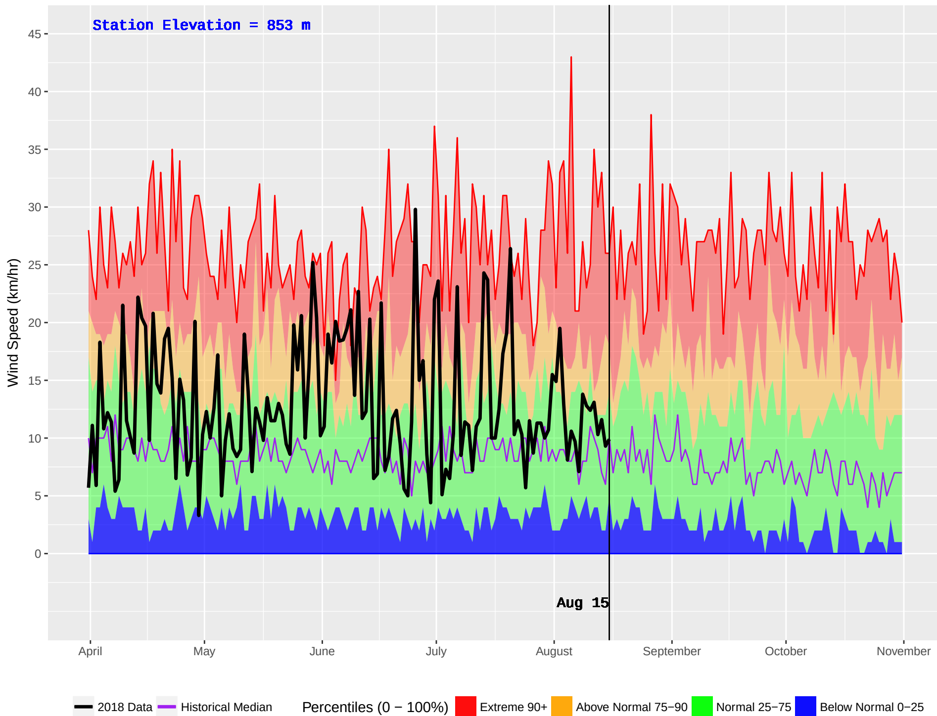
JOHNSON LAKE (419) : Historical (1986–2016) and Current (2018) Daily Wind Speed
